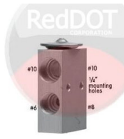
71R8321 OE#: 329-403
